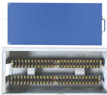
Junction Box (4TP) ME-JB-02
